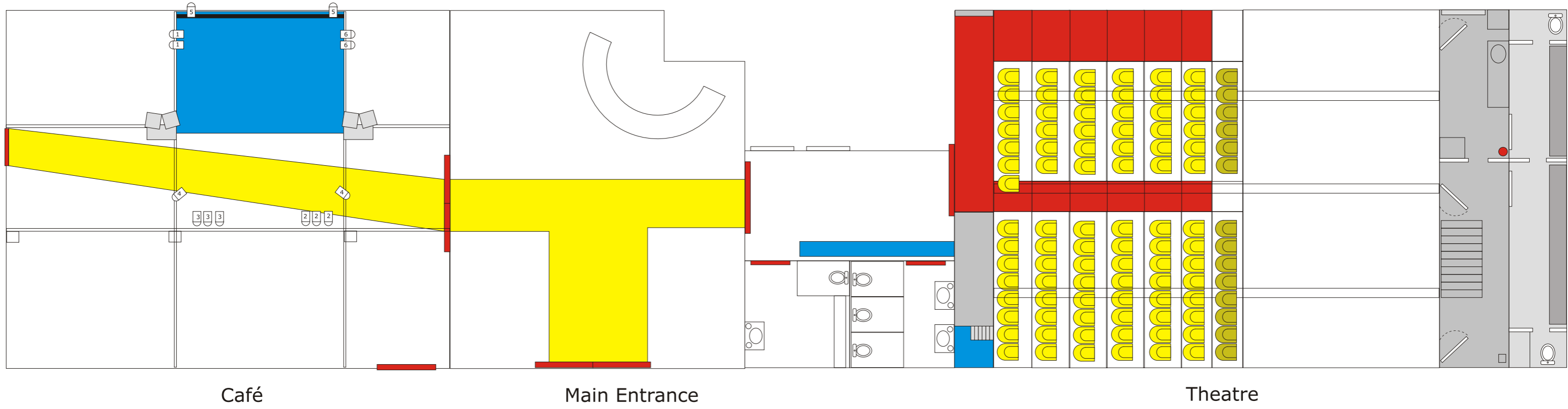
Krudttønden total plan. Drawing is not to scale
